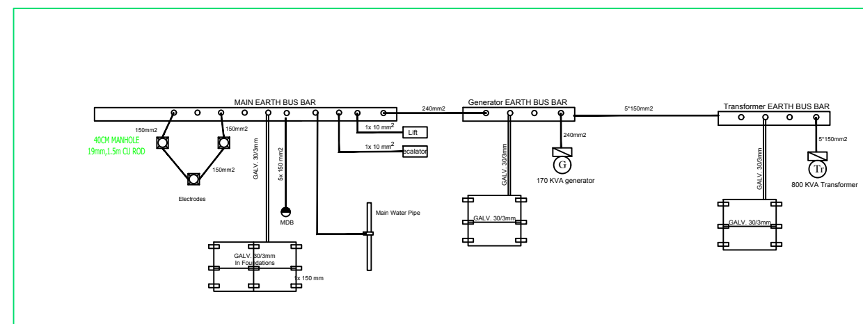
Earthing System Block Diagram
