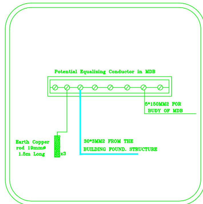
MAIN EARTH BUS BAR IN MDB
