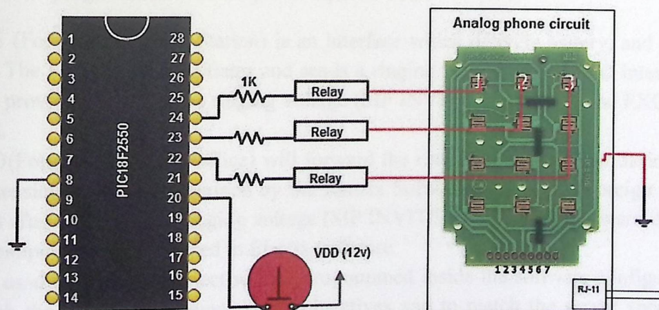
Figure 3.5: Customized Intercom
