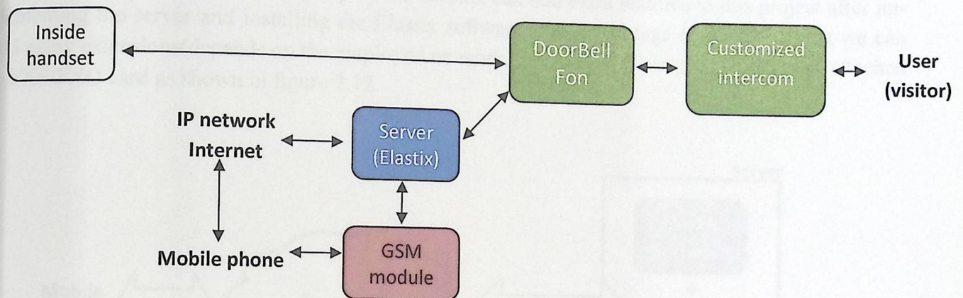
Figure 3.11: System block diagram
