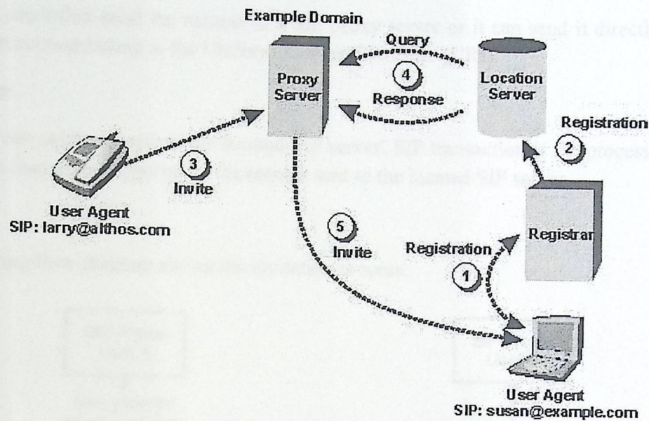
Figure 2.5: SIP operation
