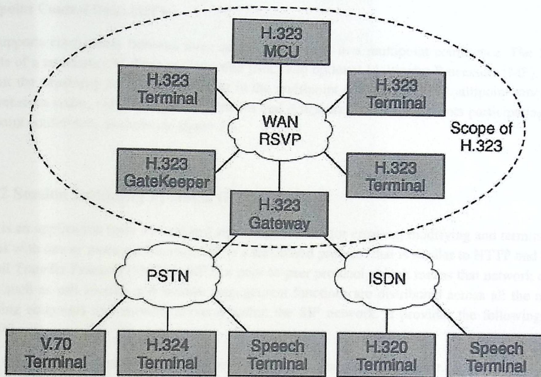
Figure 2.3: H.323 architecture
