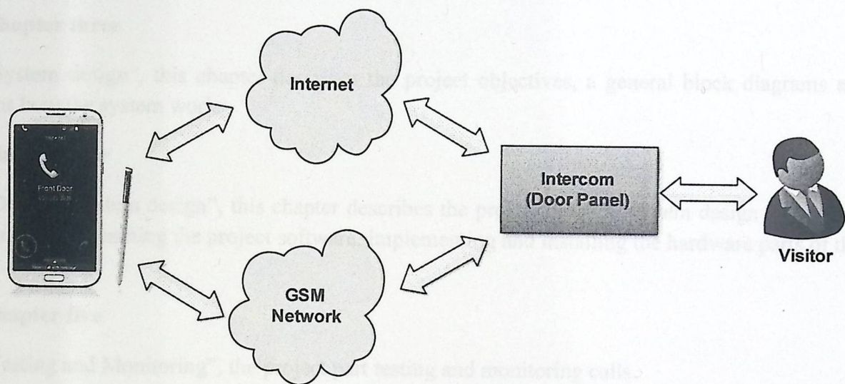
Figure 1.3: General block diagram
