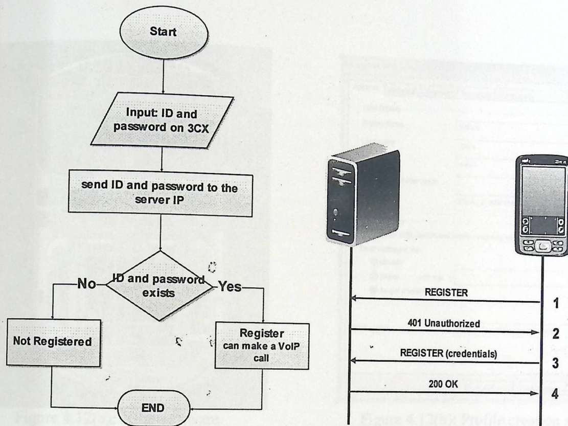
Figure 4.11: Profile authentication flowchart
