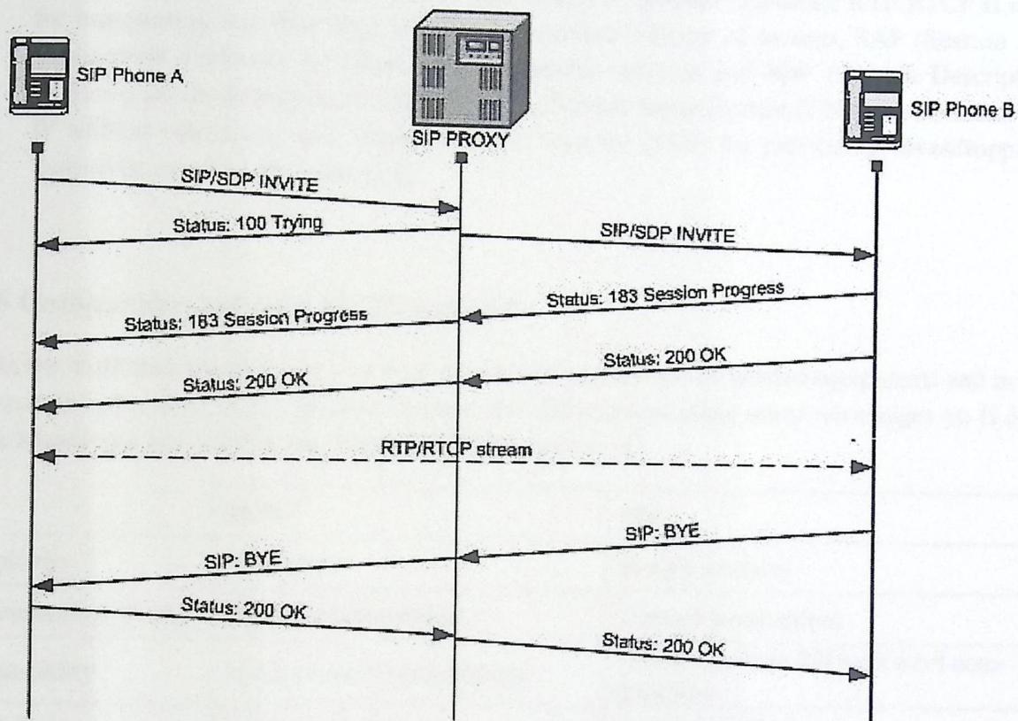
Figure 2.8: SIP Call Flow diagram
