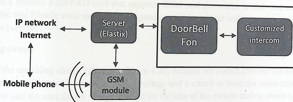
Figure 4.16: Through GSM (option 2)
