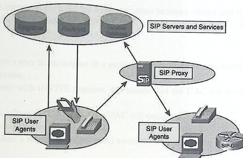
Figure 2.4: SIP system elements
