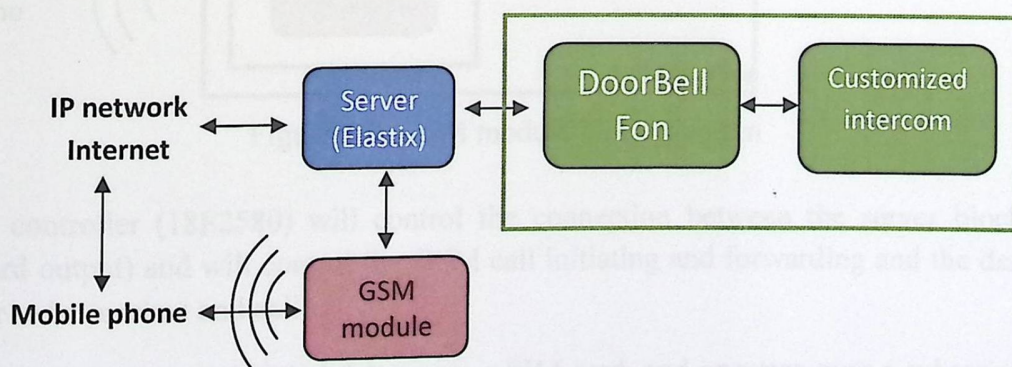
Figure 3.8: Through GSM (option 2)
