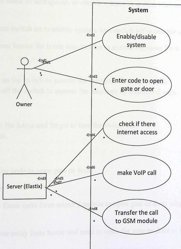
Figure 3.10: use-case diagram
