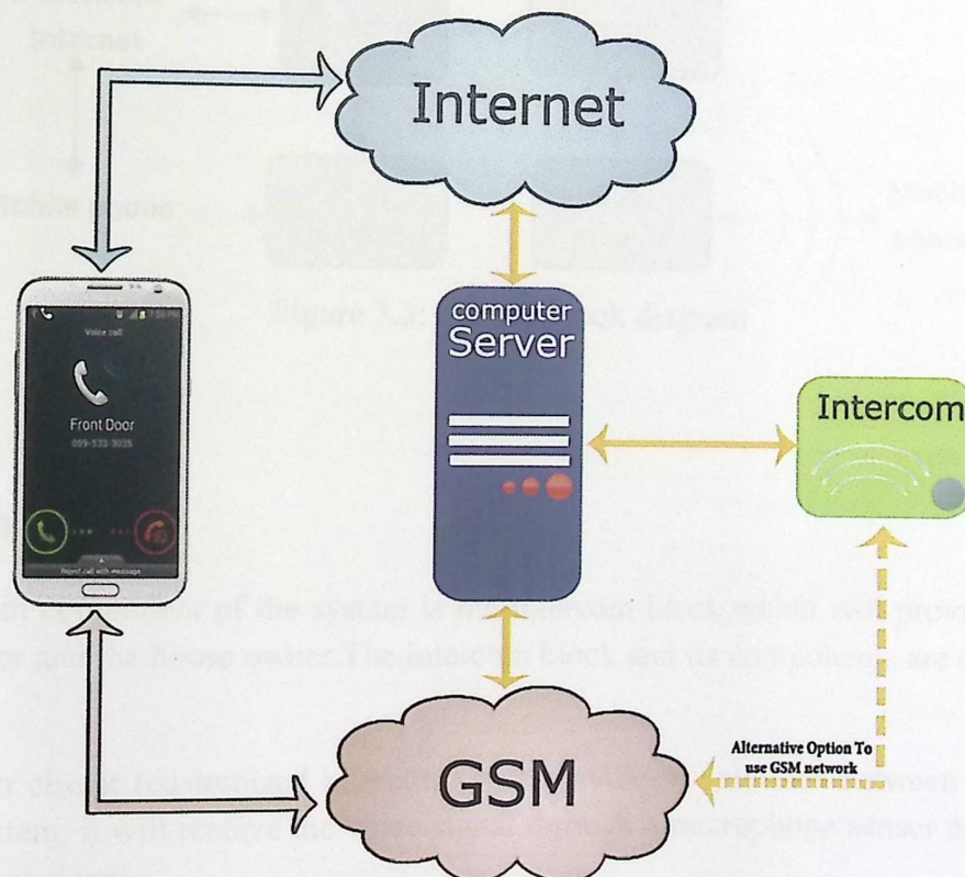
Figure 3.2: System Behavior
