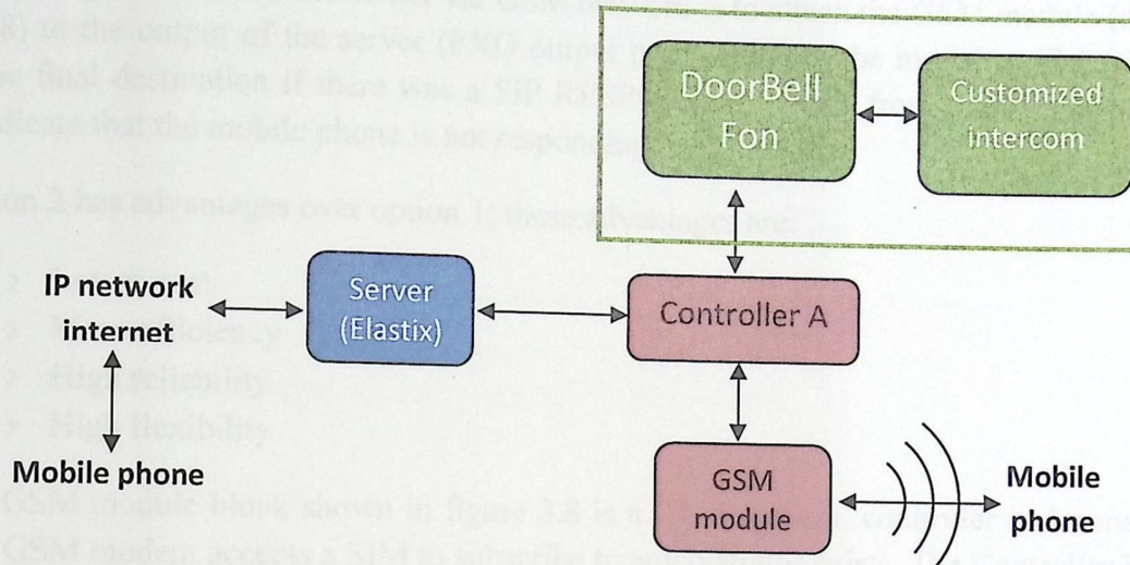
Figure 3.7: Through GSM (option 1)
