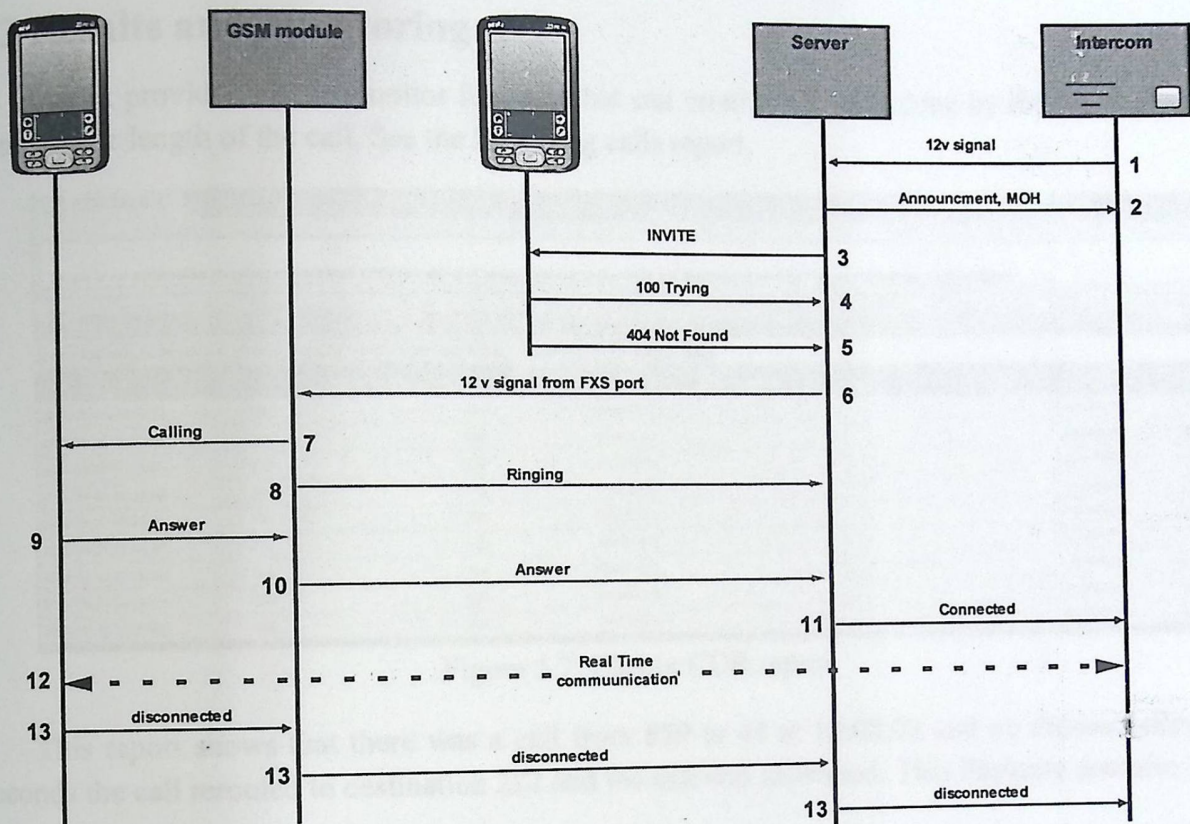
Figure 5.6: Scenario 2 call flow
