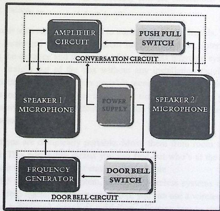
Figure 2.1: intercom system block diagram
