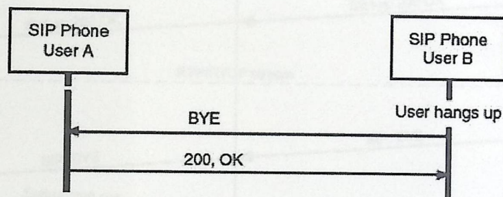
Figure 2.7: SIP session termination
