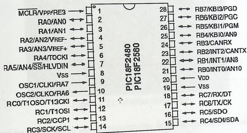
Figure 4.20: PIC18F2580 controller
