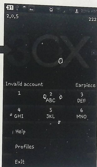
Figure 4.10(b): Settings
