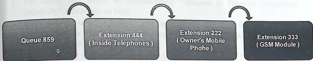
Figure 5.4: Follow-Me process
