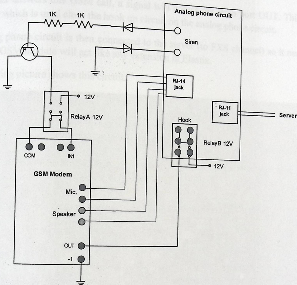
Figure 4.18: Matching circuit
