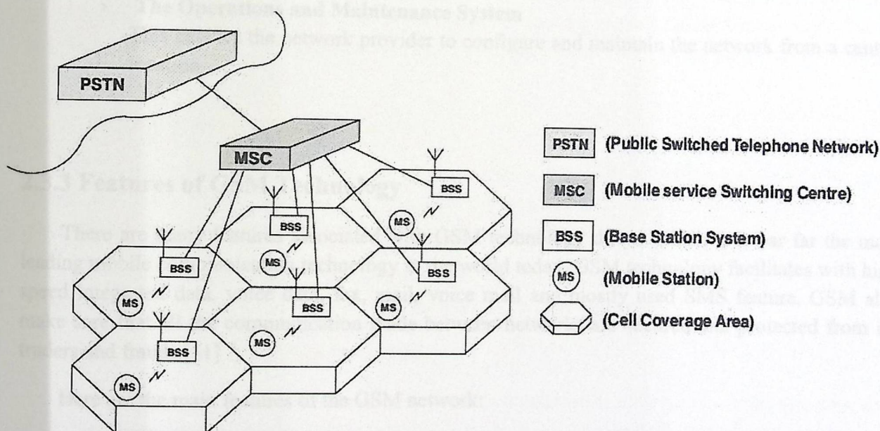
Figure 2.9: GSM network component
