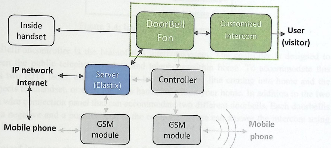
Figure 3.3: System block diagram
