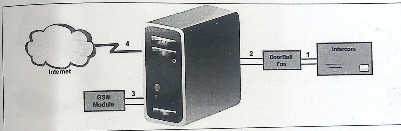
Figure 4.24: System Connections
