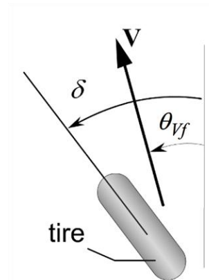
Figure 2.5 Tire slip-angle
