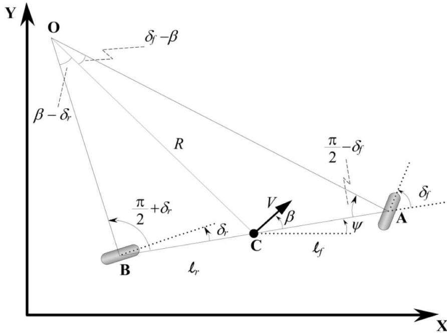
Figure 2.3: Kinematics of lateral vehicle motion
