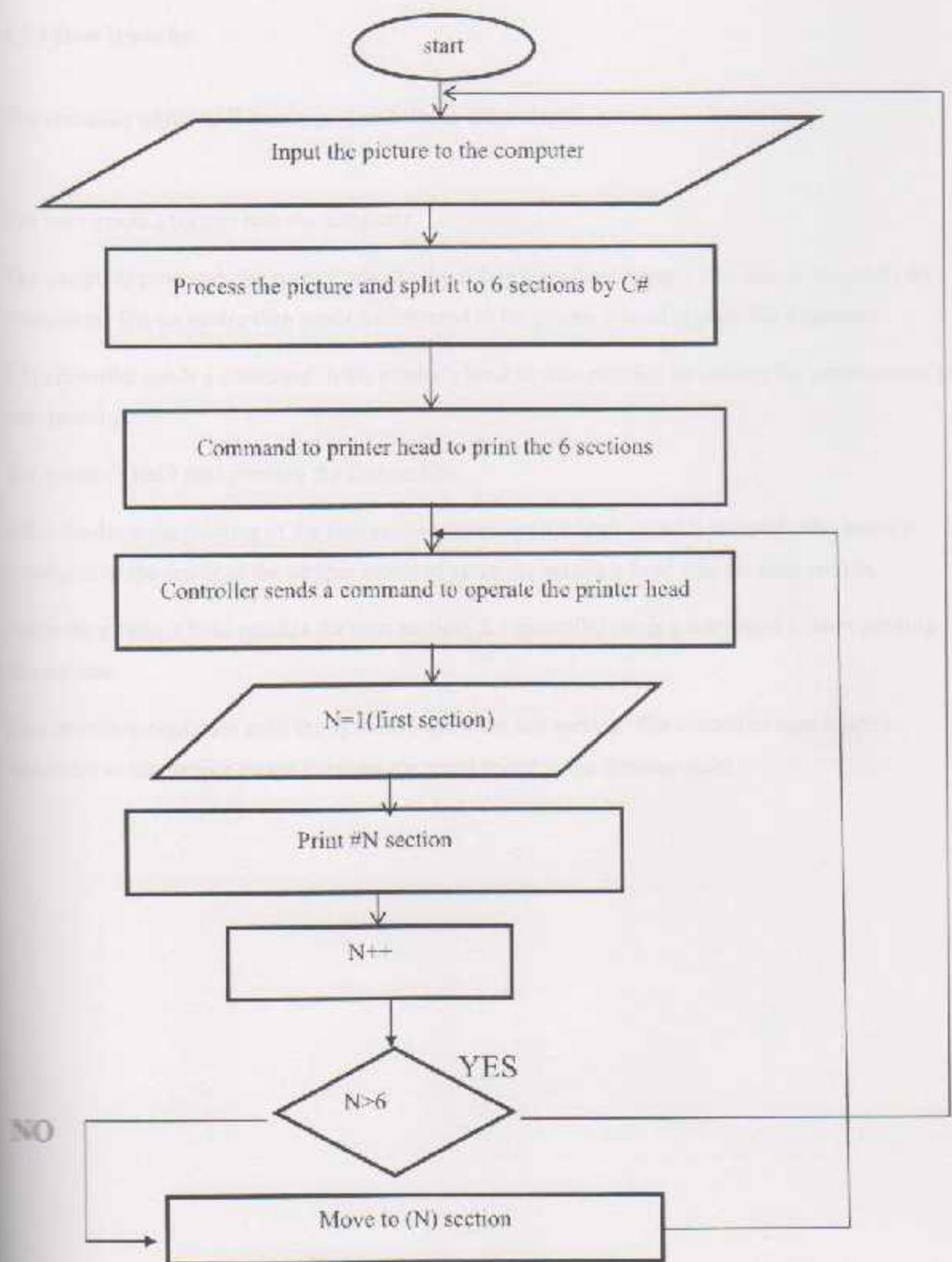
Figure 3.17: Flow chart
