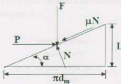
Figure 4.3: lead angle [12]
