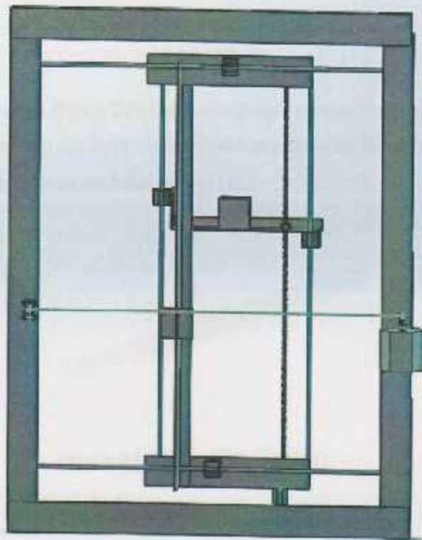
Figure 3.1: main frame
