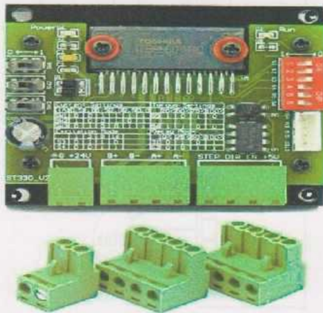
Figure 2.10: Stepper motor driver [9]
