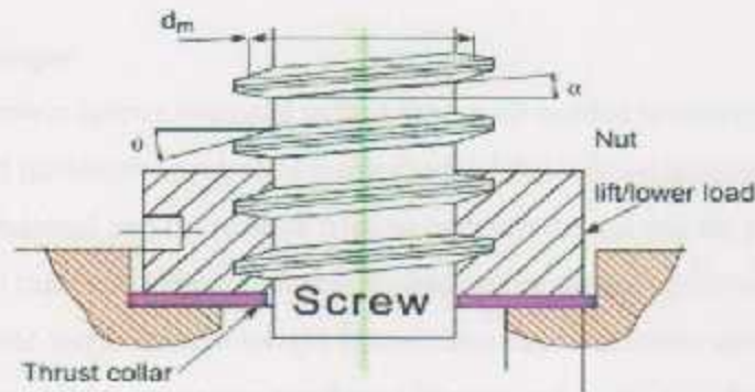
Figure 4.1: power screw
