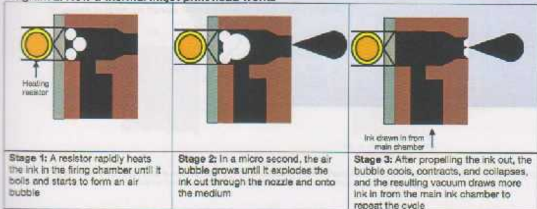
Figure 2.3: thermal printer head [5]
