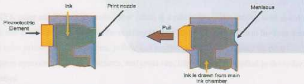
Diagram 1: How an Epson Micro Piezo™ print head works
