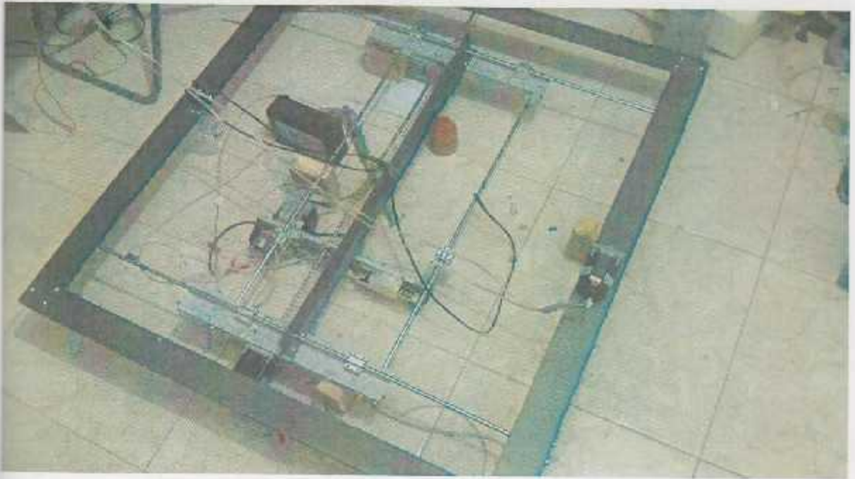
Figure 5.12: Installation the frame of X-axis
