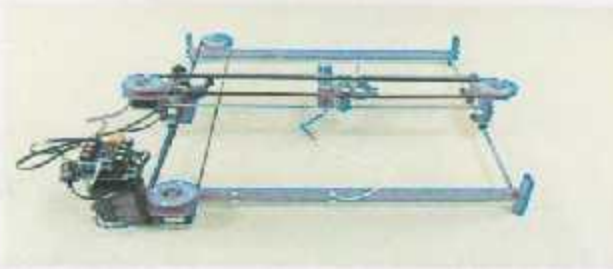
Figure 1.1: X, Yplotter [1]
