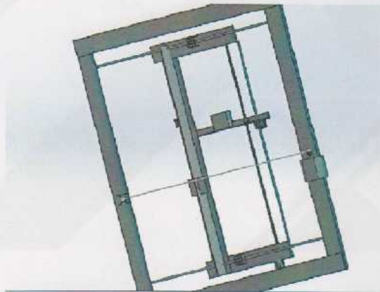
Figure 3.18: Frame layout
