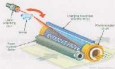
Figure 2.1: Laser printer
