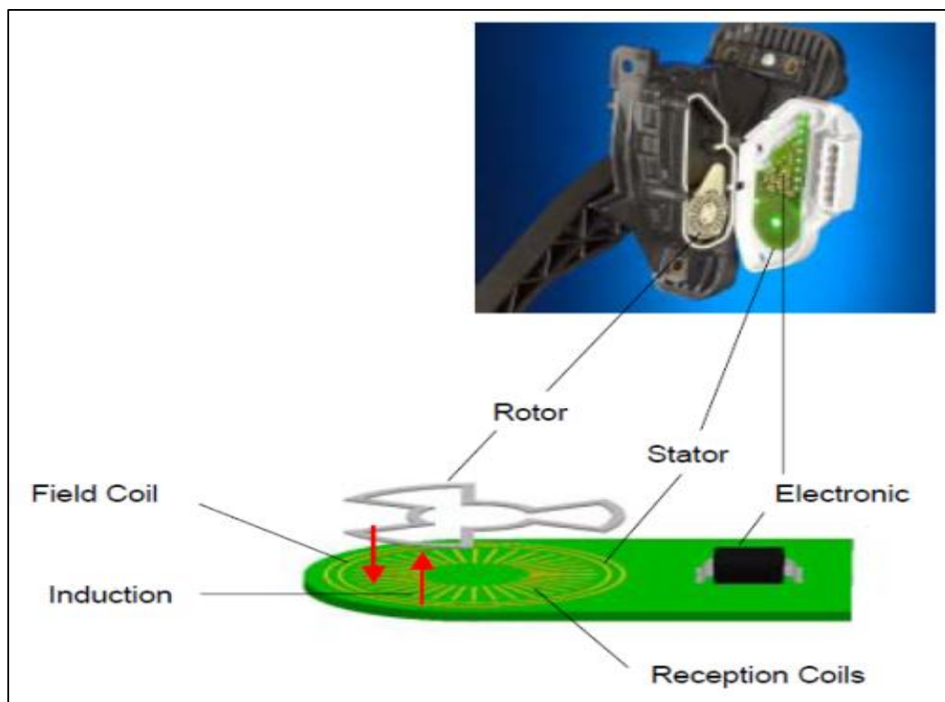
Figure 2.9: Inductive APP sensor construction
