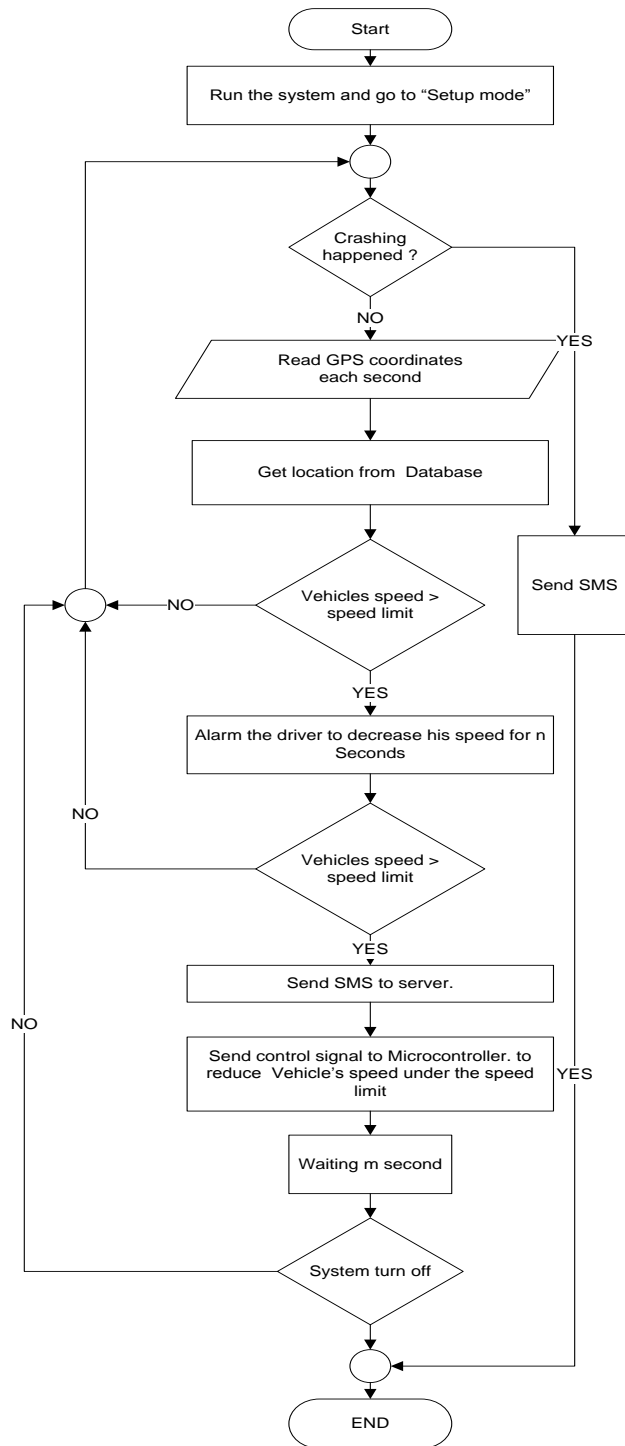
Figure 3.7: System Flowchart
