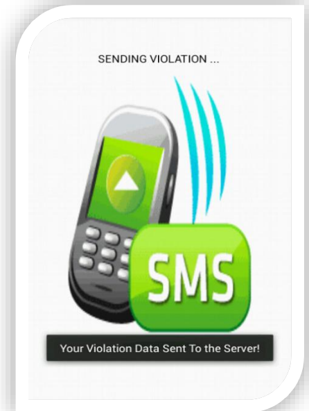
Figure 5.17: SMS activity
