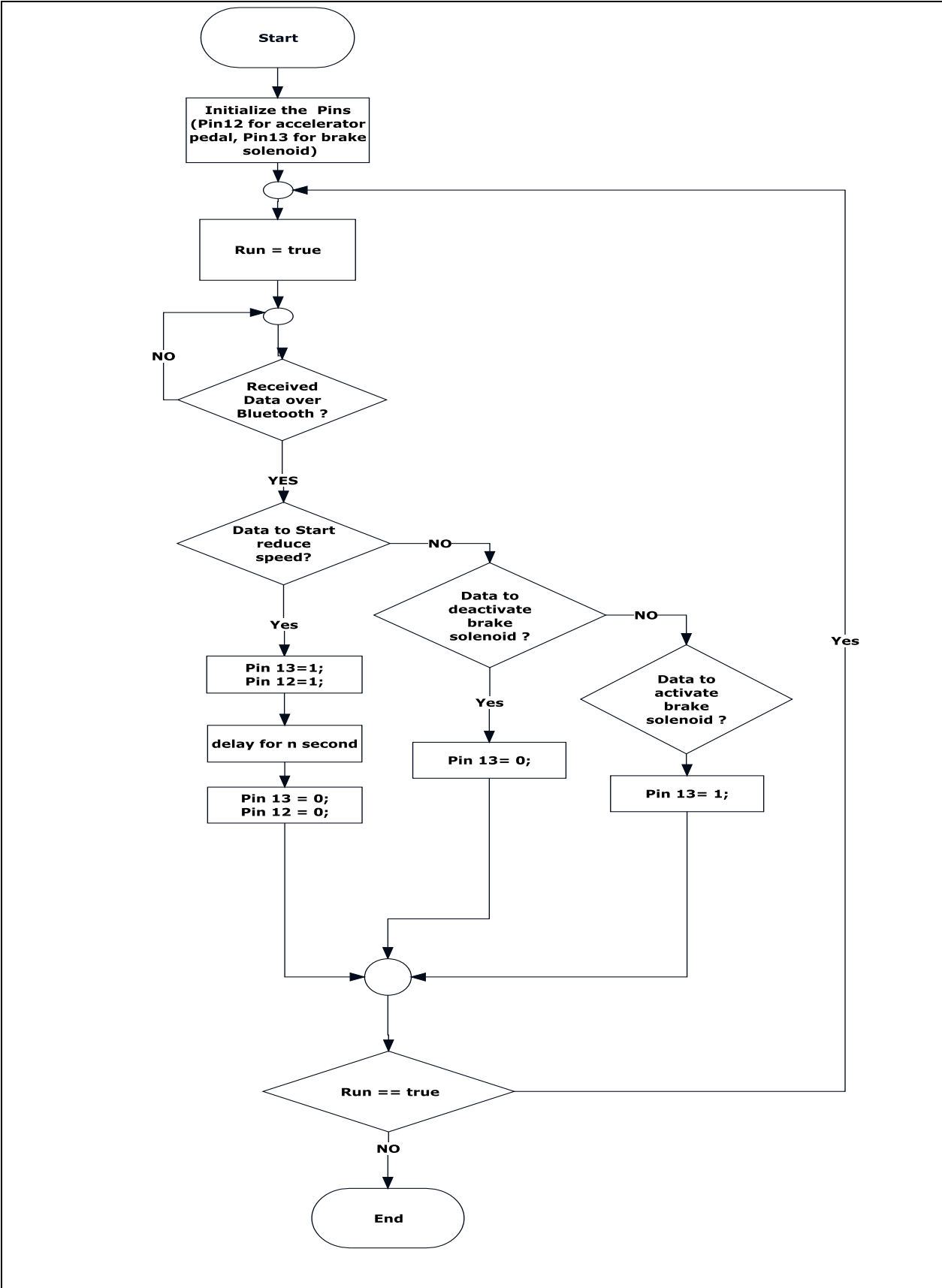
Figure 3.10:Arduino Flow Chart
