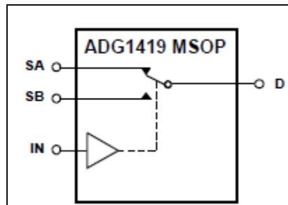
Figure 4.23: Functional block diagram
