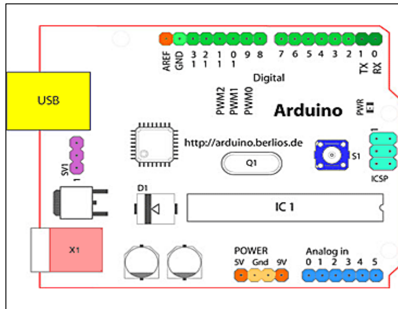
Figure 2.6: Arduino board components
