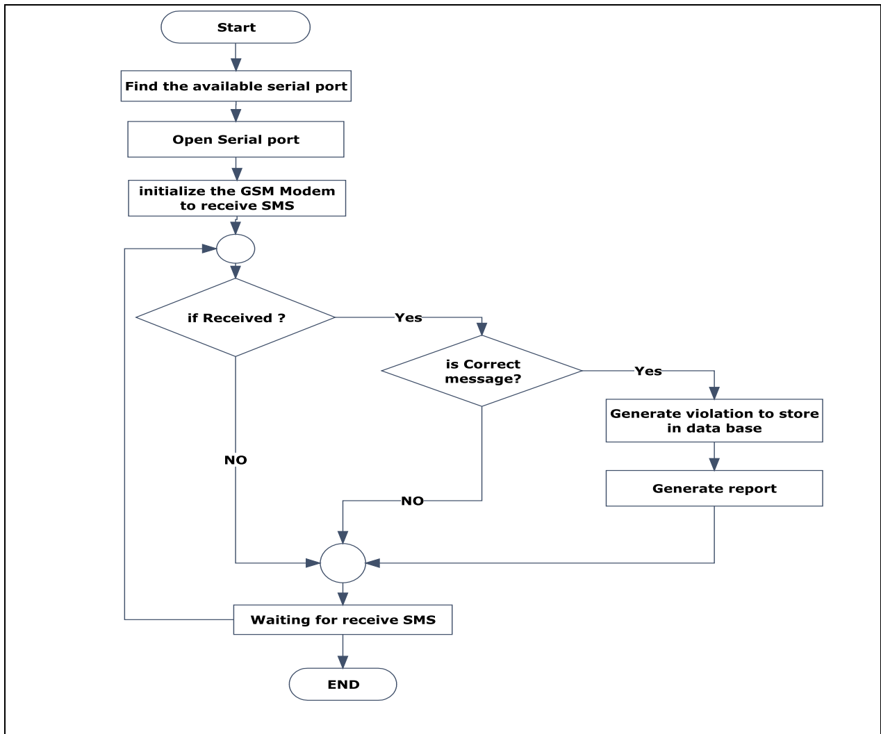
Figure 3.12:Server receiving violation flow chart
