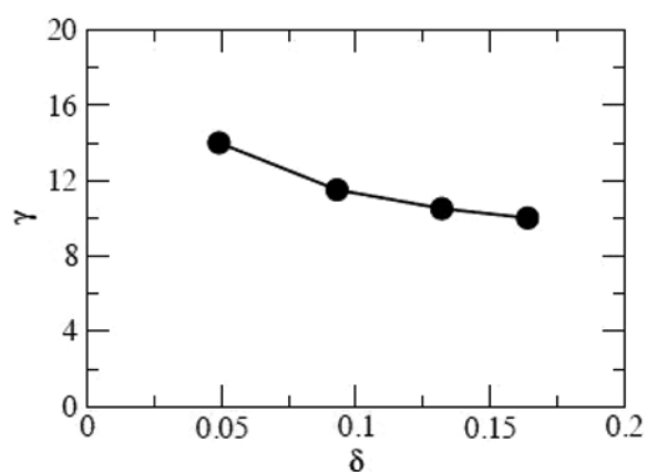
Figure 5. Reduction of minimum amounts of surfactant, \tilde{\sigma} , needed for solubilizing 10 wt. % of water in diesel by adding the co-surfactant C_{16-18}E_{140} .
