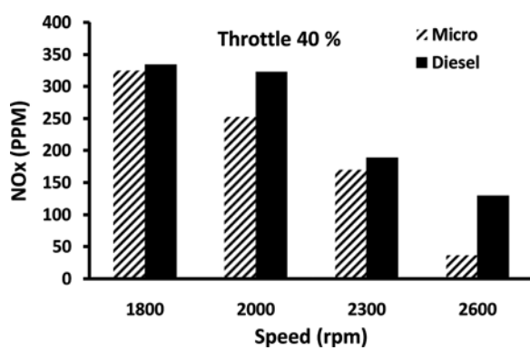
Figure 9. NO x levels as a function of engine speed at constant 40% throttle.
