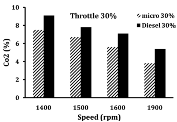
Figure 12. CO 2 levels as a function of engine speed at constant 30% throttle.
