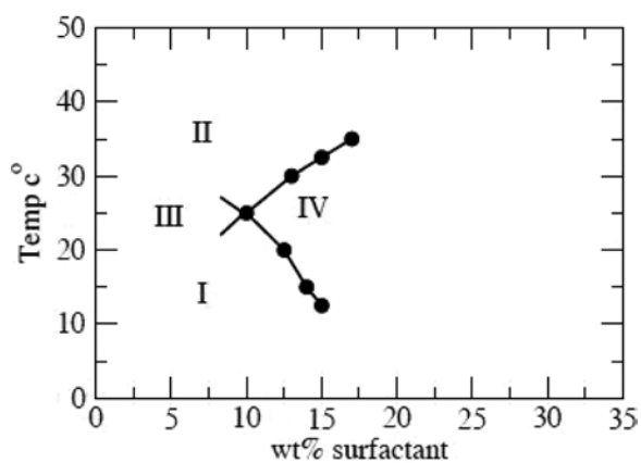
Figure 1. Phase diagram of water-heptane- C_{11}E_3 at water to heptane wt. ratio of 1:1 with C_{16-18}E_{140} at \delta=0.10 .
