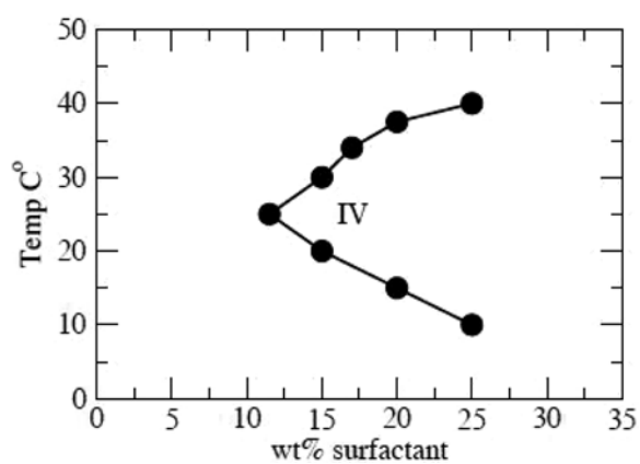
Figure 2. Phase diagram of water-diesel- C_{11}E_3 at water to diesel wt. ratio of 1:1 with C_{16} - _{18}E_{140} at \delta=0.10 .
