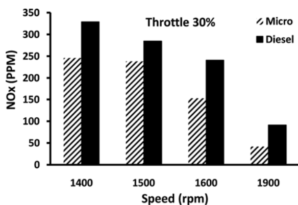
Figure 8. NO x levels as a function of engine speed at constant 30% throttle.
