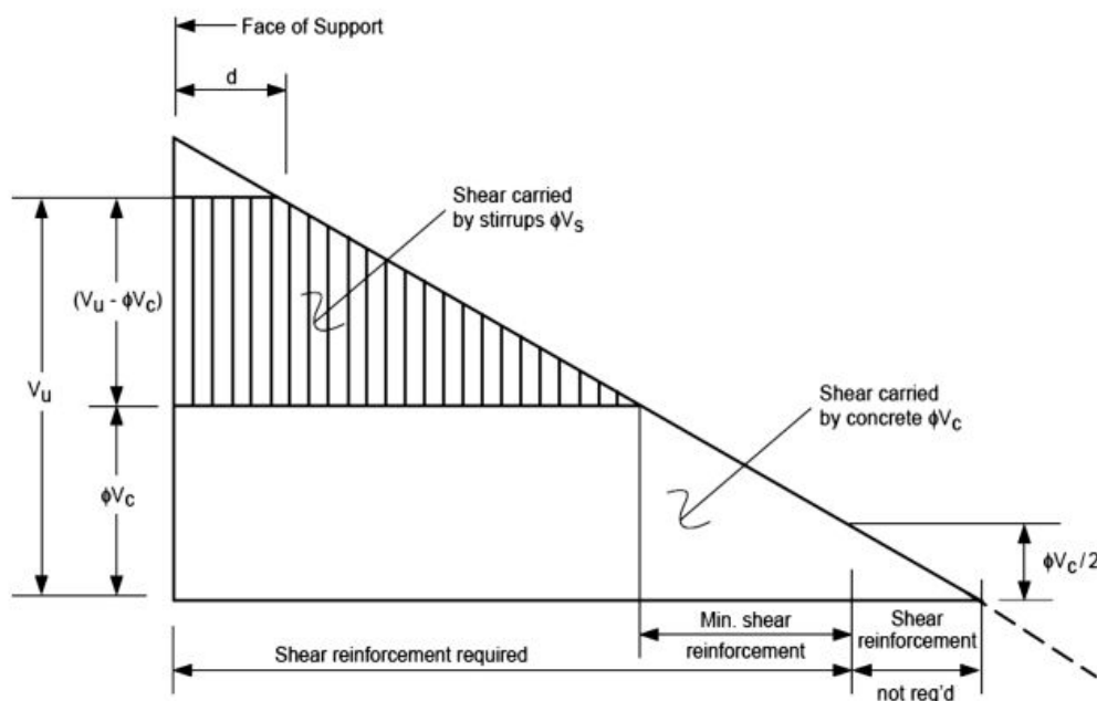
Figure (4-10) Shear diagonal.
