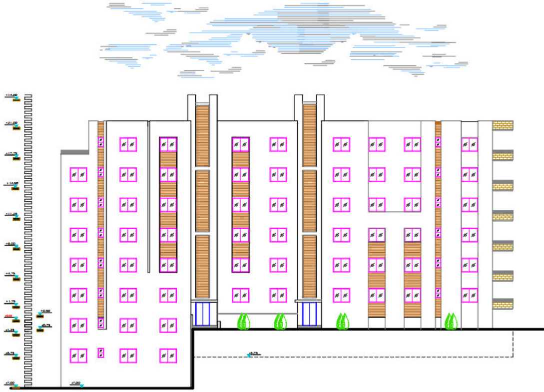
East Elevation
