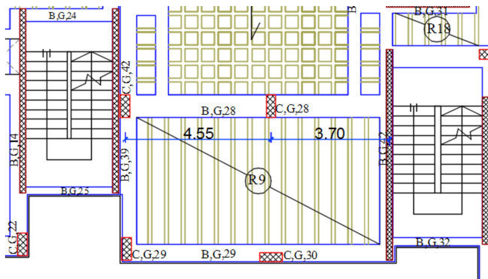
Figure (4-12) location of Beam (B.G.28) in slab drawing plan.
