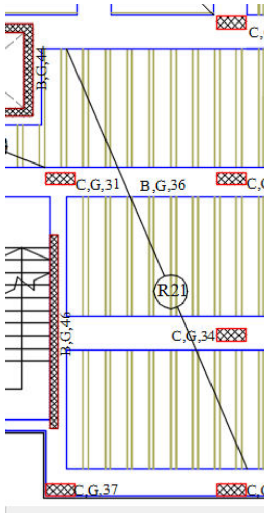
Figure (4-7) location of Rib (R21) in slab drawing plan.
