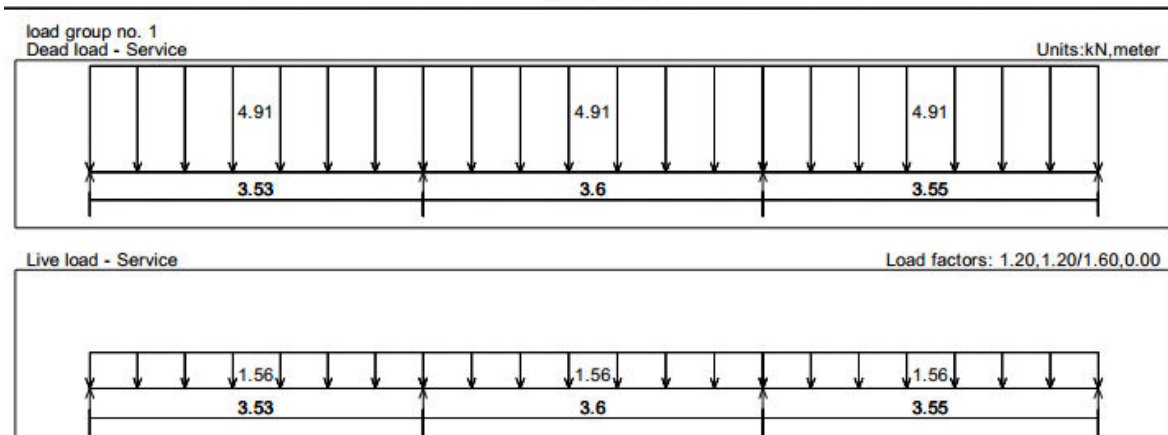
Figure (4-8) shows rib geometry and loads.
