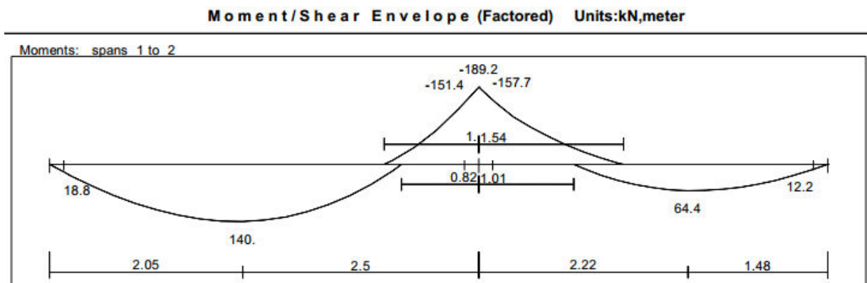
Figure (4-17) Envelope moment diagram for Beam (B.G.21).
