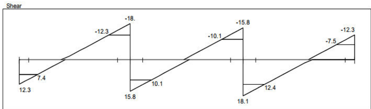
Figure (4-11) Shear envelop diagram.
