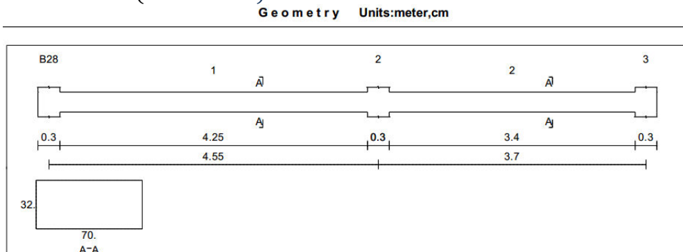
Figure (4-13) Beam (B.G.21) geometry.
