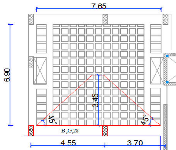
Figure (4-15) trapezoidal load on beam (B.G.28)
