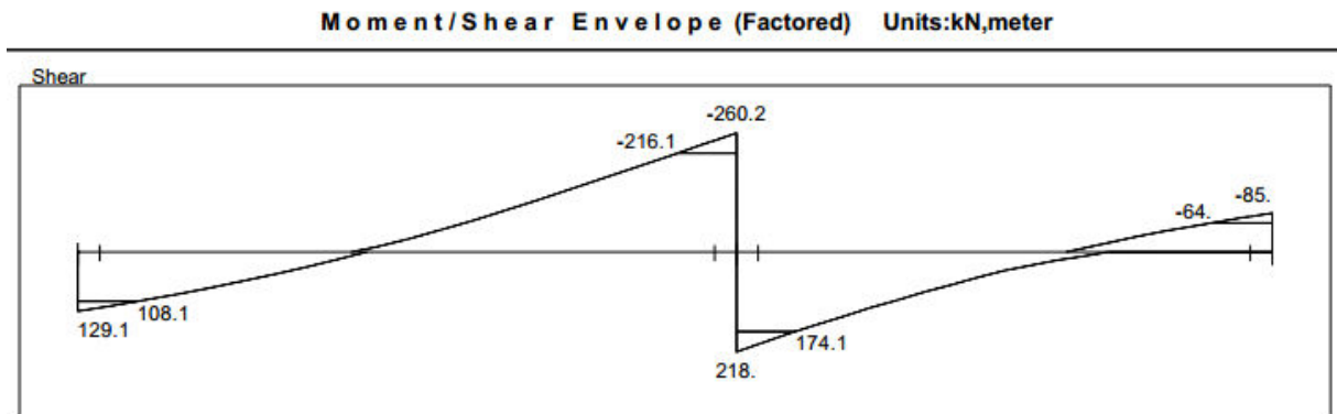
Figure (4-18) Shear envelop diagram of Beam.
