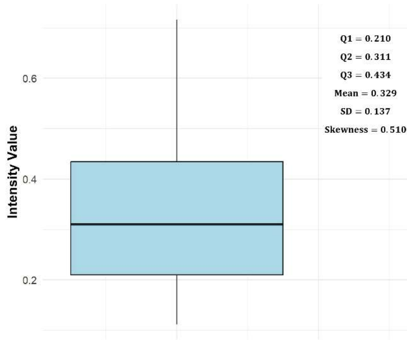
Figure 2: Boxplot of the SAR dataset showing the skewness and key descriptive statistics. The figure includes quartiles ( Q1 = 0.210 , Q2 = 0.311 , Q3 = 0.434 ), mean ( 0.329 ), standard deviation ( 0.137 ), and skewness ( 0.510 ).
