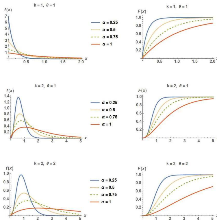
Figure 1: PDF (left) and CDF (right) curves of the UD fractional Gamma distribution for varying \alpha , \theta , and k . The plots highlight the flexibility of the distribution as parameters change.
