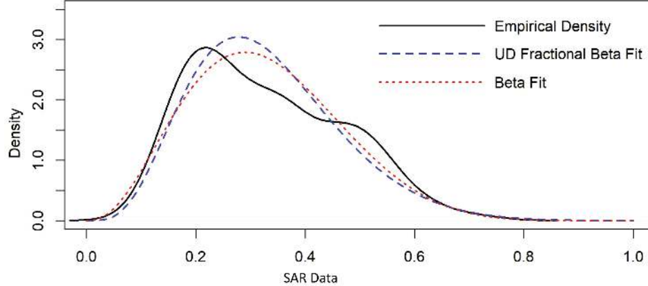
Figure 3: Empirical density function of the data overlaid with the fitted PDFs of the UD fractional Beta and classical Beta distributions.
