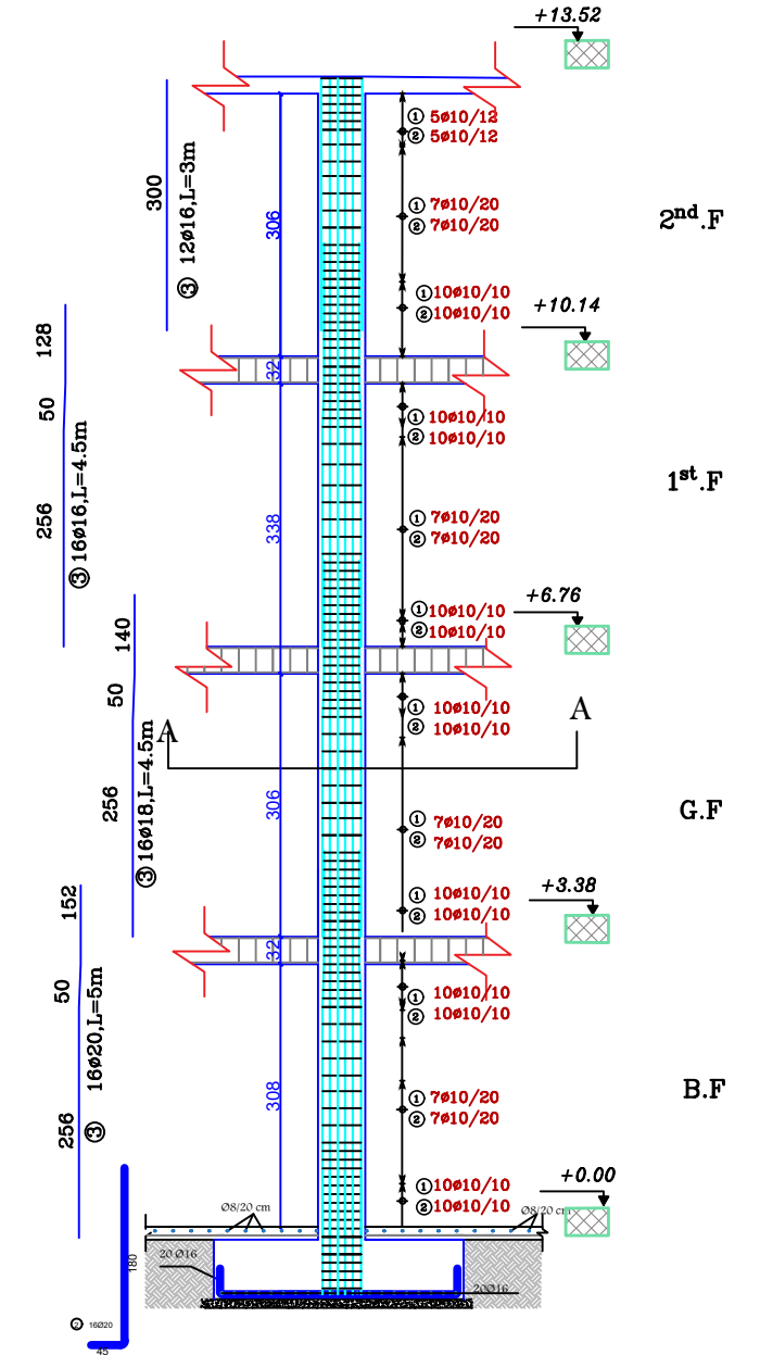
Columns detailing's (G3) SCALE 1:50
