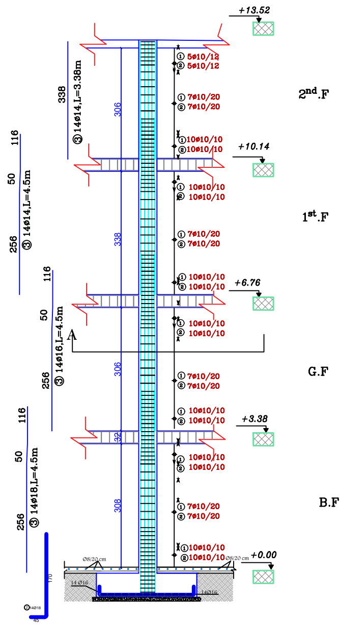
Columns detailing's (G2) SCALE 1:50
