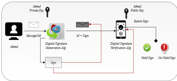
Figure 9. DSA Process [23].
