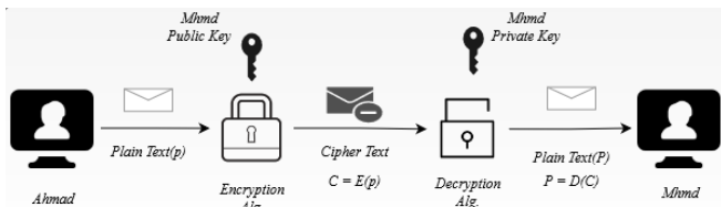
Figure 5. RSA Process [18].
