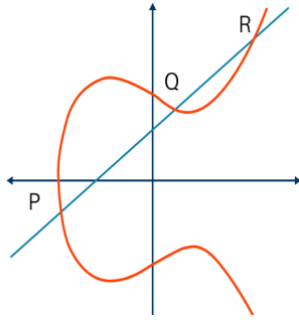
Figure 8. ECC Basics [22].
