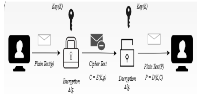
Figure 11. DES Algorithm [30].
