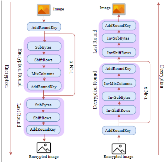
Figure 12. AES Algorithm [31].
