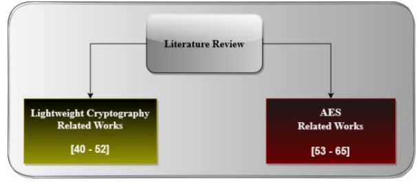
Figure 13. Literature Review
