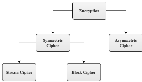
Figure 4. Encryption Models [9].
