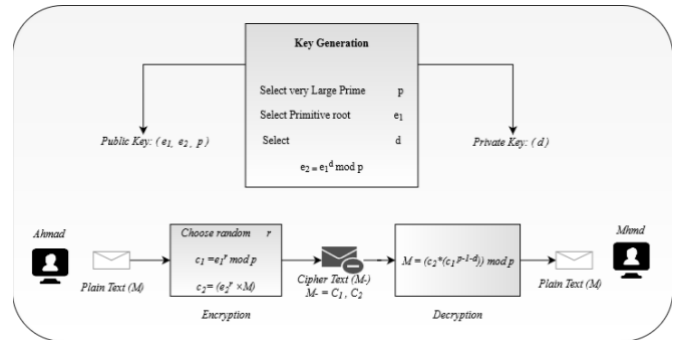
Figure 6. ElGamal Alg. [20].
