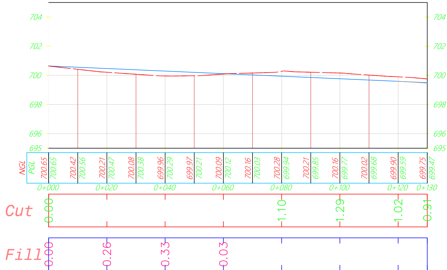
AL15, FROM STA 0+000 TO. 0+130
