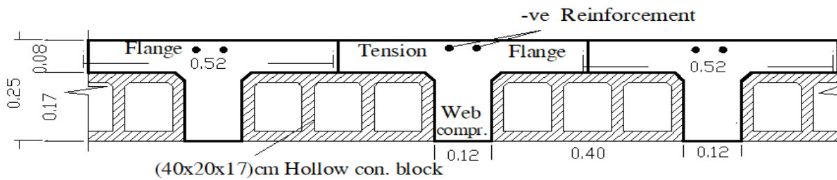
Rib section at supports or at cantilevers
