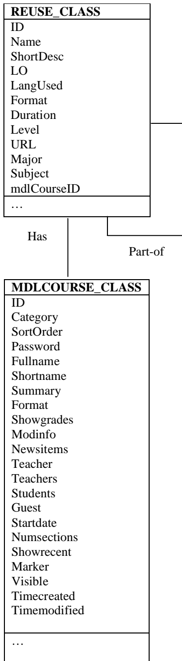
Figure 2. UML Conceptual Schema for REUSE_CLASS and MDLCOURSE_CLASS
