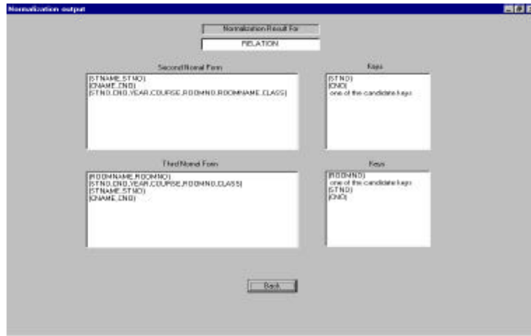
Fig. 2: Output relations from the normalization process
