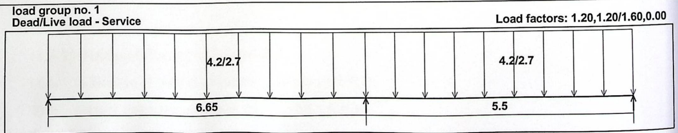
(Figure (4-4) : loading of Rib (A0-R1)
