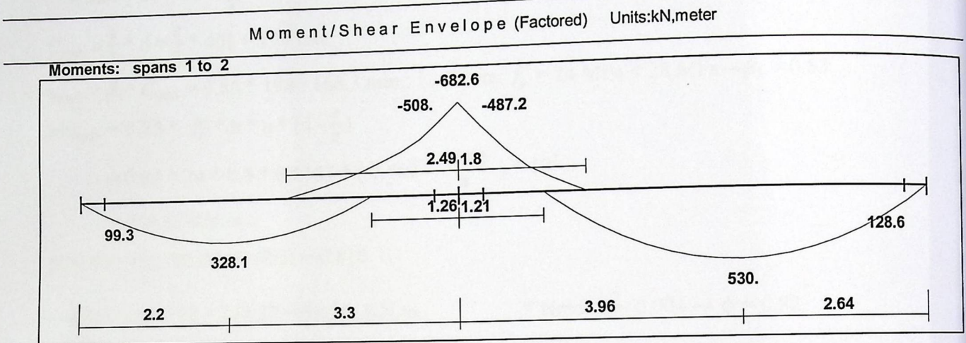
Figure (4-9) : Moment Envelop for Beam (A0-B37)
