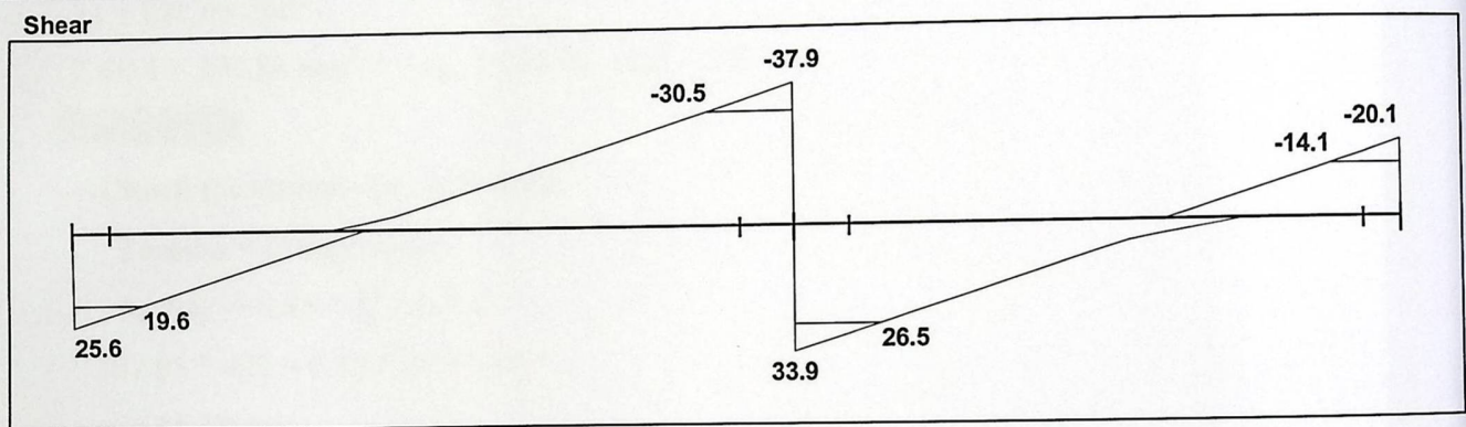
Figure (4-6) : Shear Envelop of rib (A0-R1)
