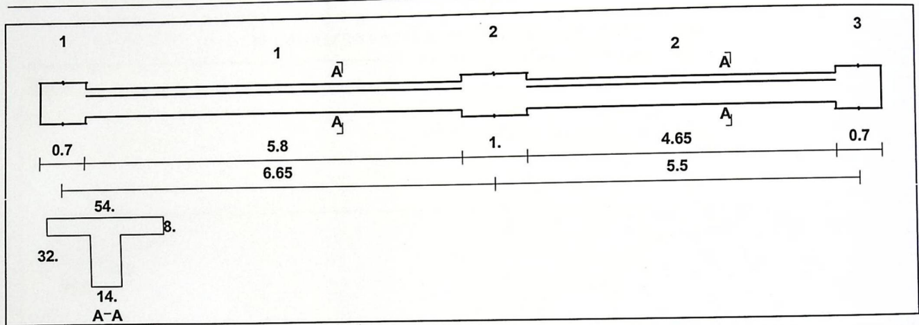
Figure (4-3): Rib geometry.
