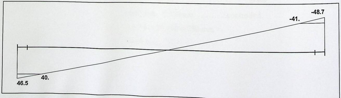
Figure(4-12) : Envelope Shear and moment Diagram of Stair
