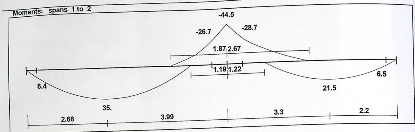
Figure (4-5) : Moment Envelop of rib (A0-R1)
