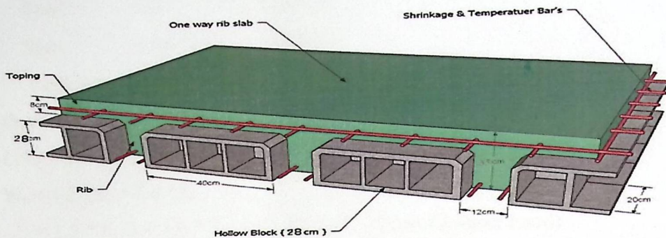
Fig. (4-2) One way rib slab
