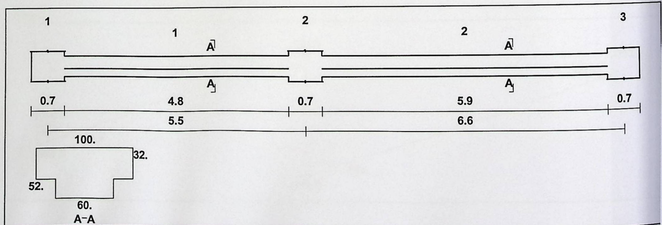
Figure (4-7) : Beam Geometry.
