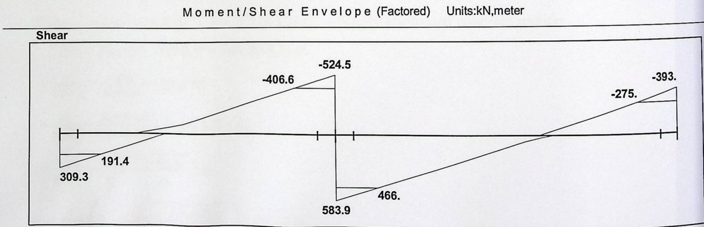
Figure (4-10) : Shear Envelop for Beam.
