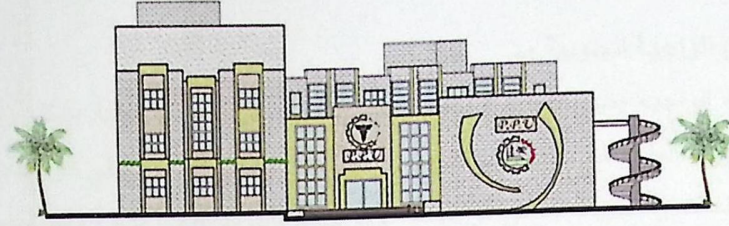
West Elevation A 09 Scale : 1/250
