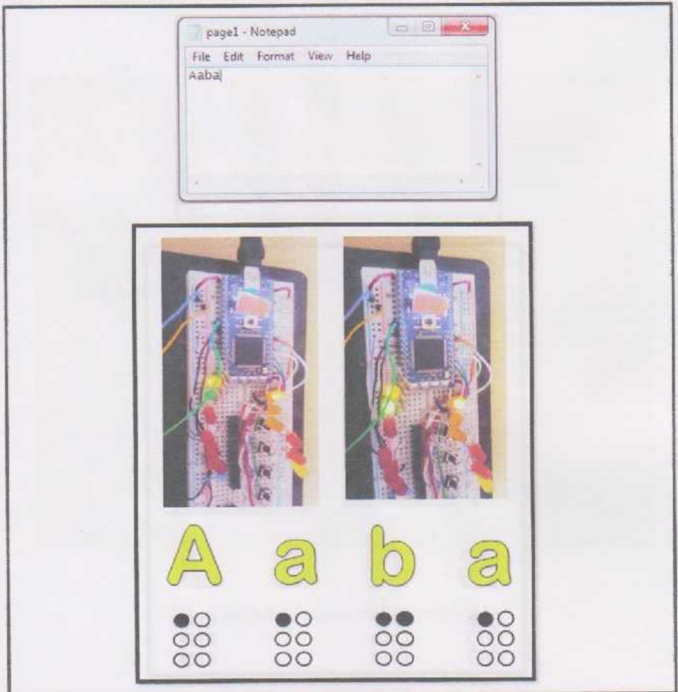
Fig. 6.5 Testing the code using twelve leds as two Braille cells –page 1-
