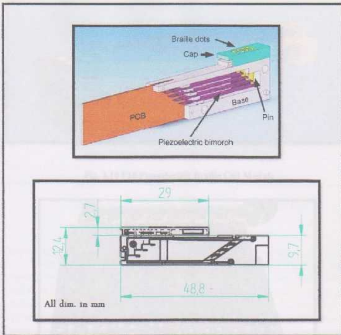
Fig. 3.9 Assembly drawing of the Piezoelectric Braille Cell
