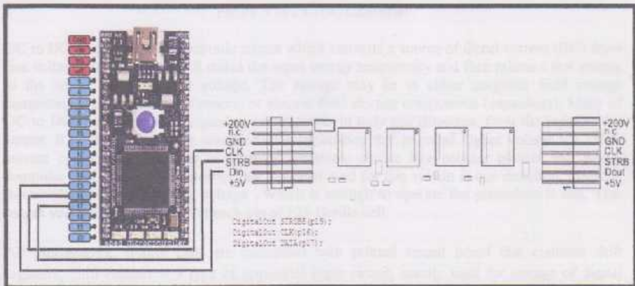
Fig. 3.13 PCB Connection with mbed microcontroller
