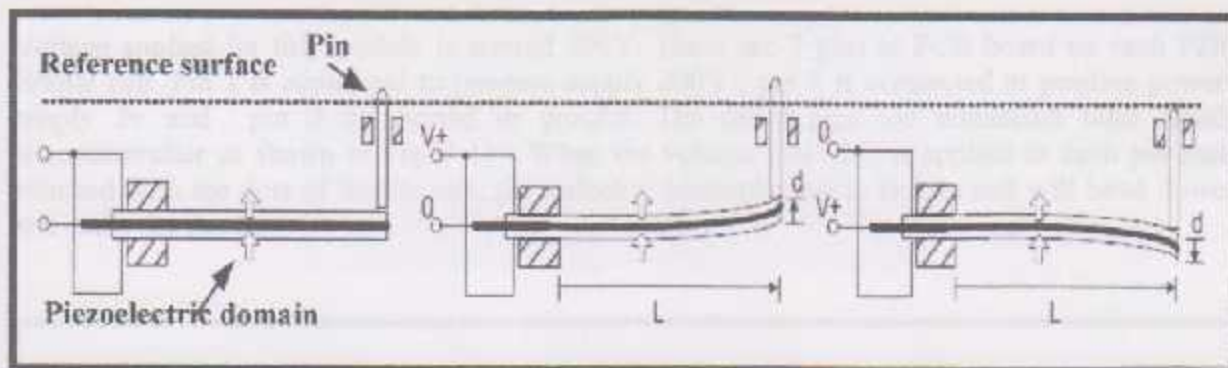
Fig. 3.12 Actuation mechanism of the Piezoelectric Braille Cell
