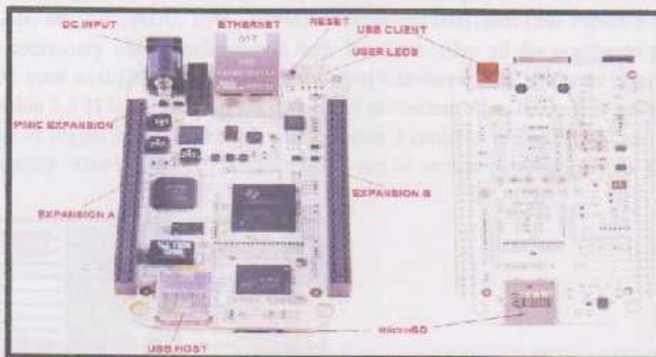
Fig. 3.6 BeagleBone board
