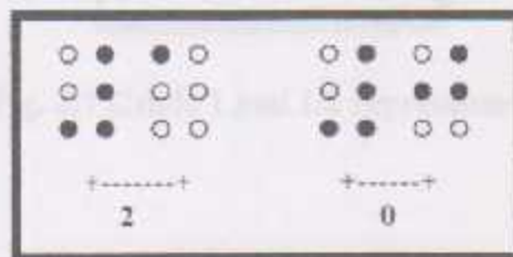
Fig. 2.5 Numbers representation
