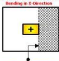
Critical section for bending moment at face of Column.
