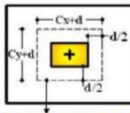
Critical Section for Two-Way Shear (Punching Action) at distance (d/2) from face of column. B_o = 2(C_x + C_y) + 4 \times d
