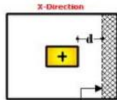
Critical Section for One-Way Shear (Beam Action) at distance (d) from face of column.
