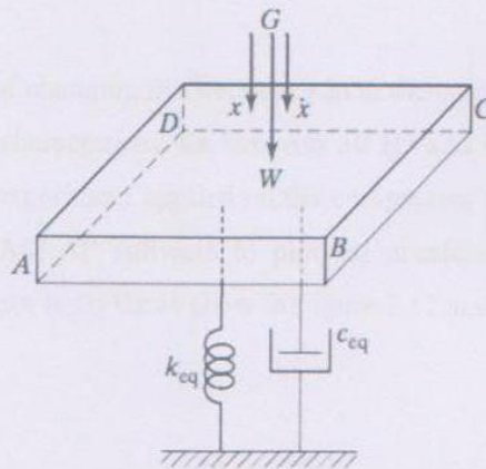
Figure 3.16 Compressor modeling equivalent.
