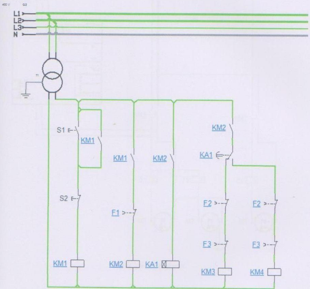
Figure 2.5 Control circuit.
