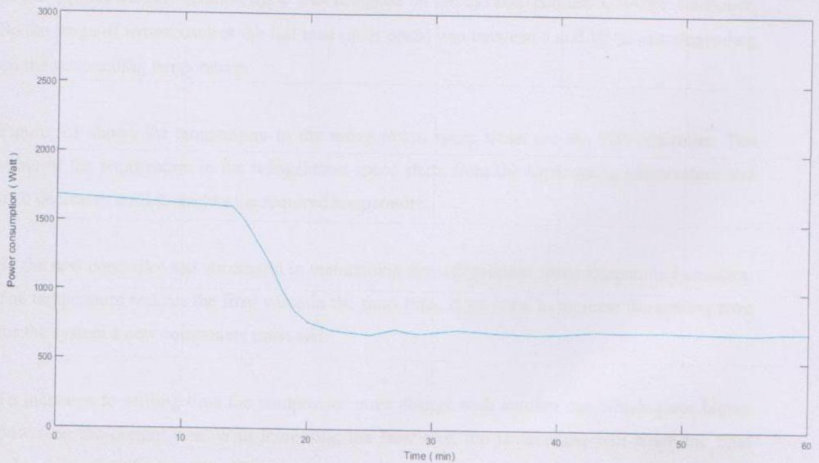
Figure 5.2 Power response with the new PID controller.
