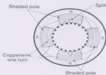
Figure 2.1 Electrical component of AC motor.
