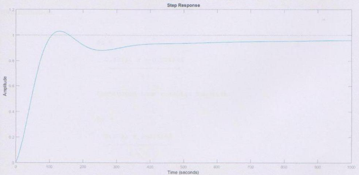
Figure 4.12 Step response.
