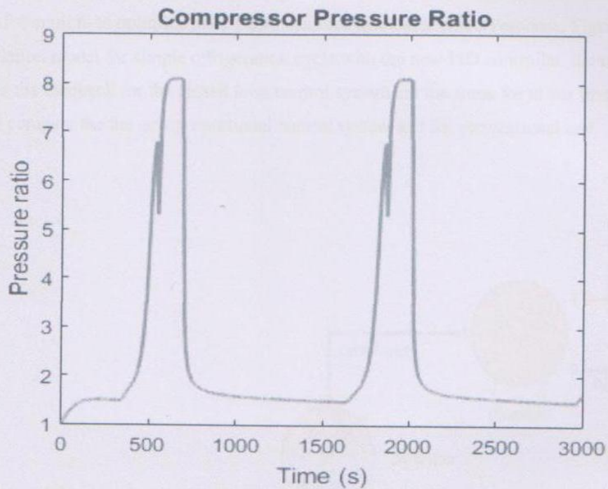
Figure 3.7 Pressure ratio of the compressor versus time.
