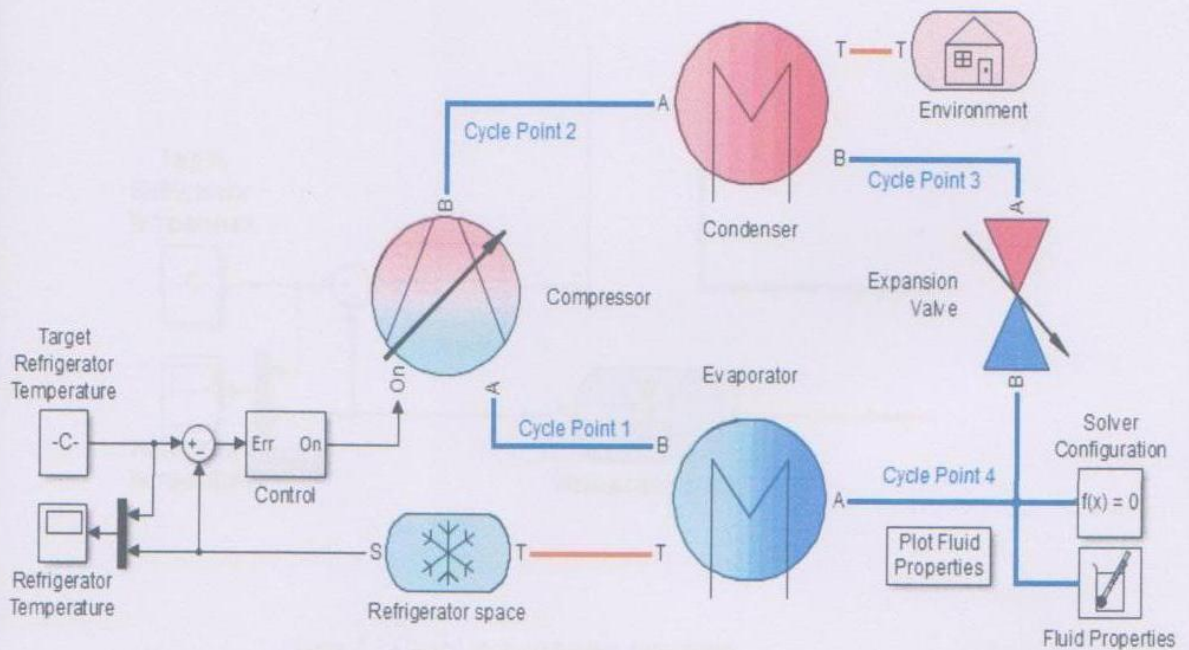
Figure 3.1 Simple vapor-compression refrigeration cycle model.
