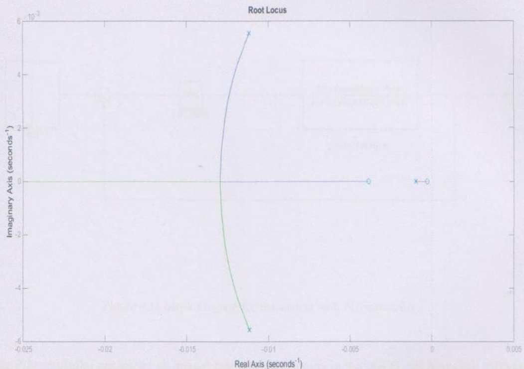
Figure 4.9 Root Locus
