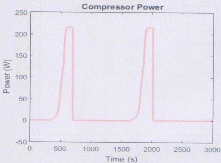
Figure 3.5 Compressor power verses time.
