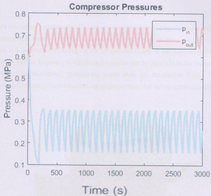
Figure 3.13 Pressure in the inlet and the outlet of the compressor versus time when using PID controller.
