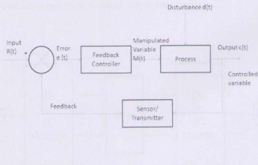
Figure 2.3 closed loop control system diagram.
