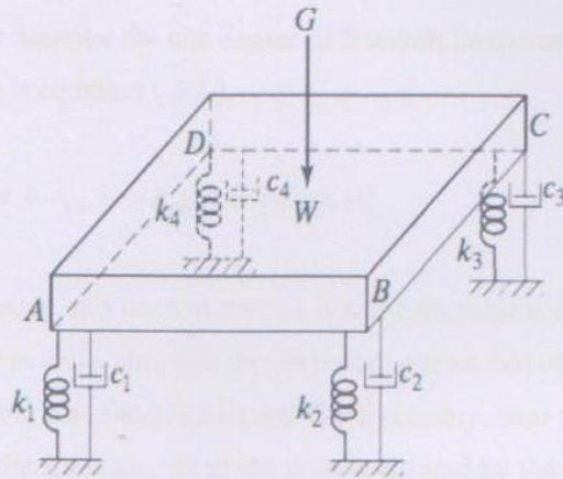
Figure 3.15 Compressor modeling.
