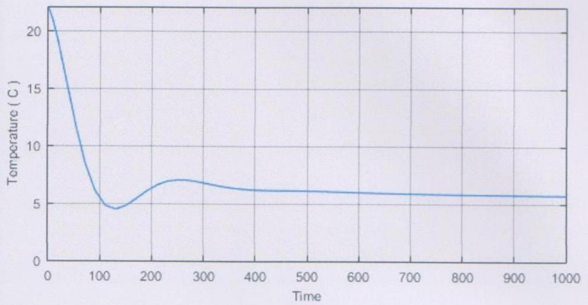
Figure 4.18 Output response.
