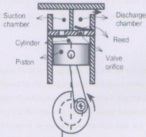
Figure 2.2 Mechanical component of reciprocating compressor.
